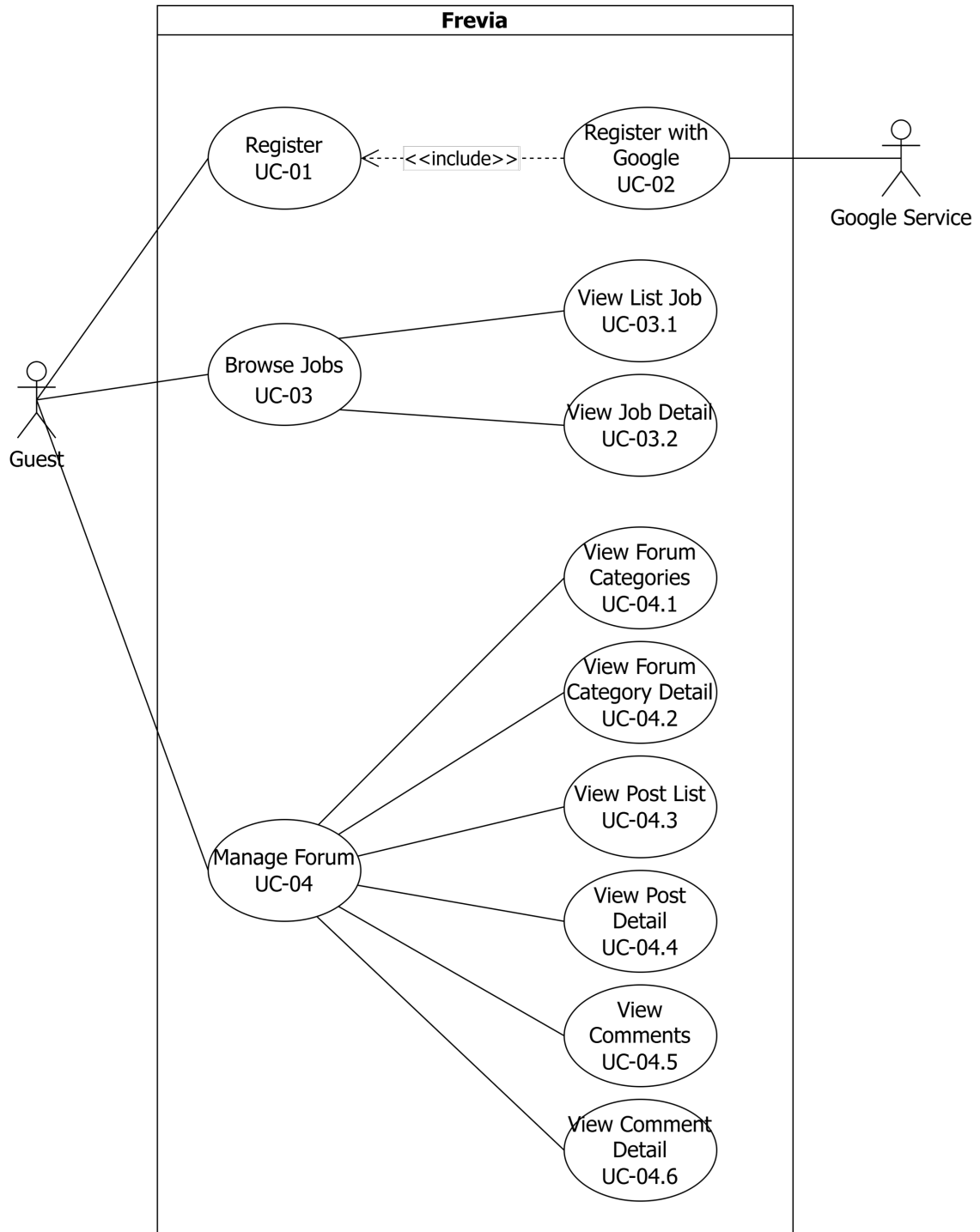
Figure 2: Guest Usecase
