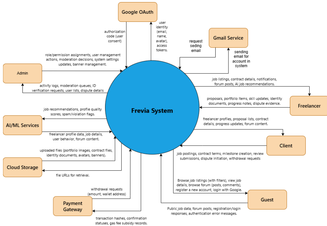
Figure 1: Context diagram
