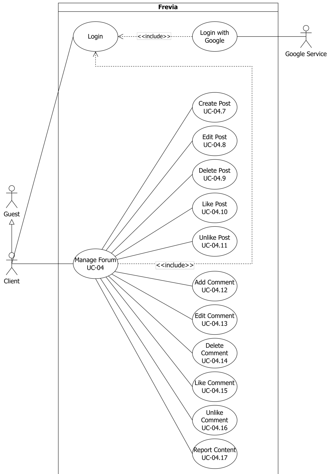
Figure 4: Client Usecase
