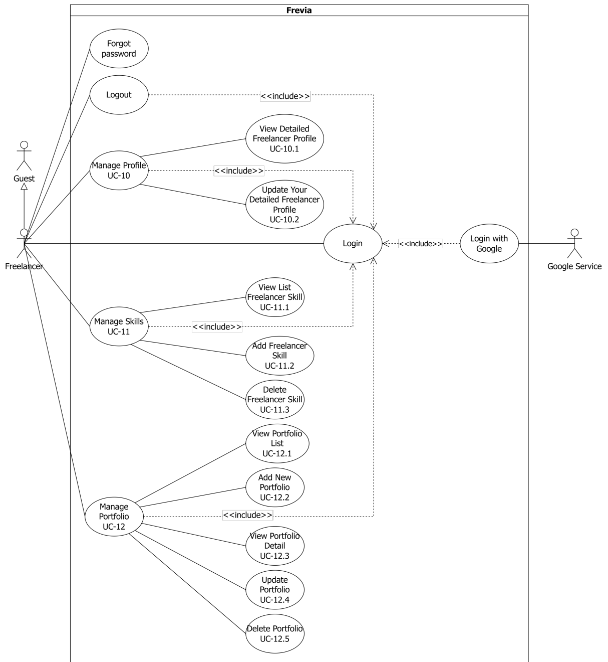
Figure 5: Freelancer Usecase
