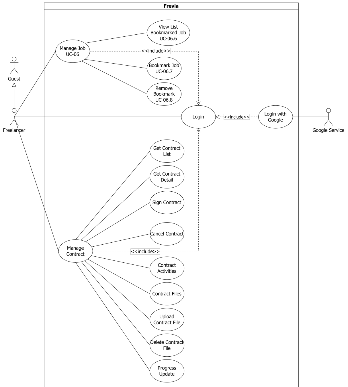
Figure 7: Freelancer Usecase
