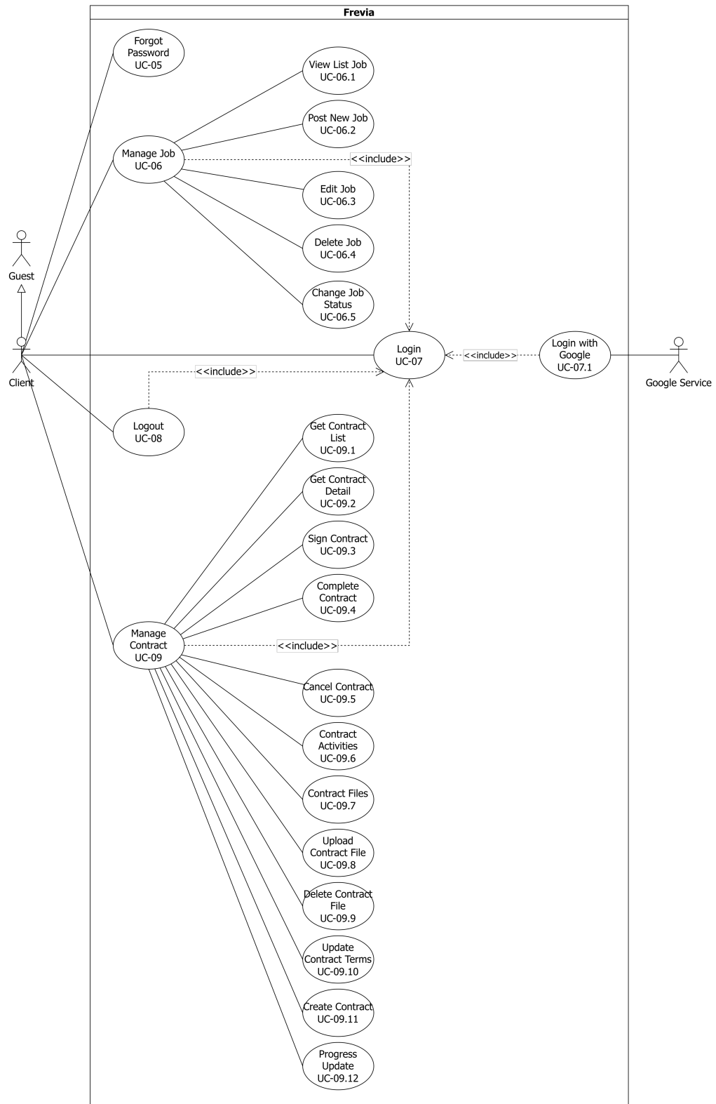
Figure 3: Client Usecase
