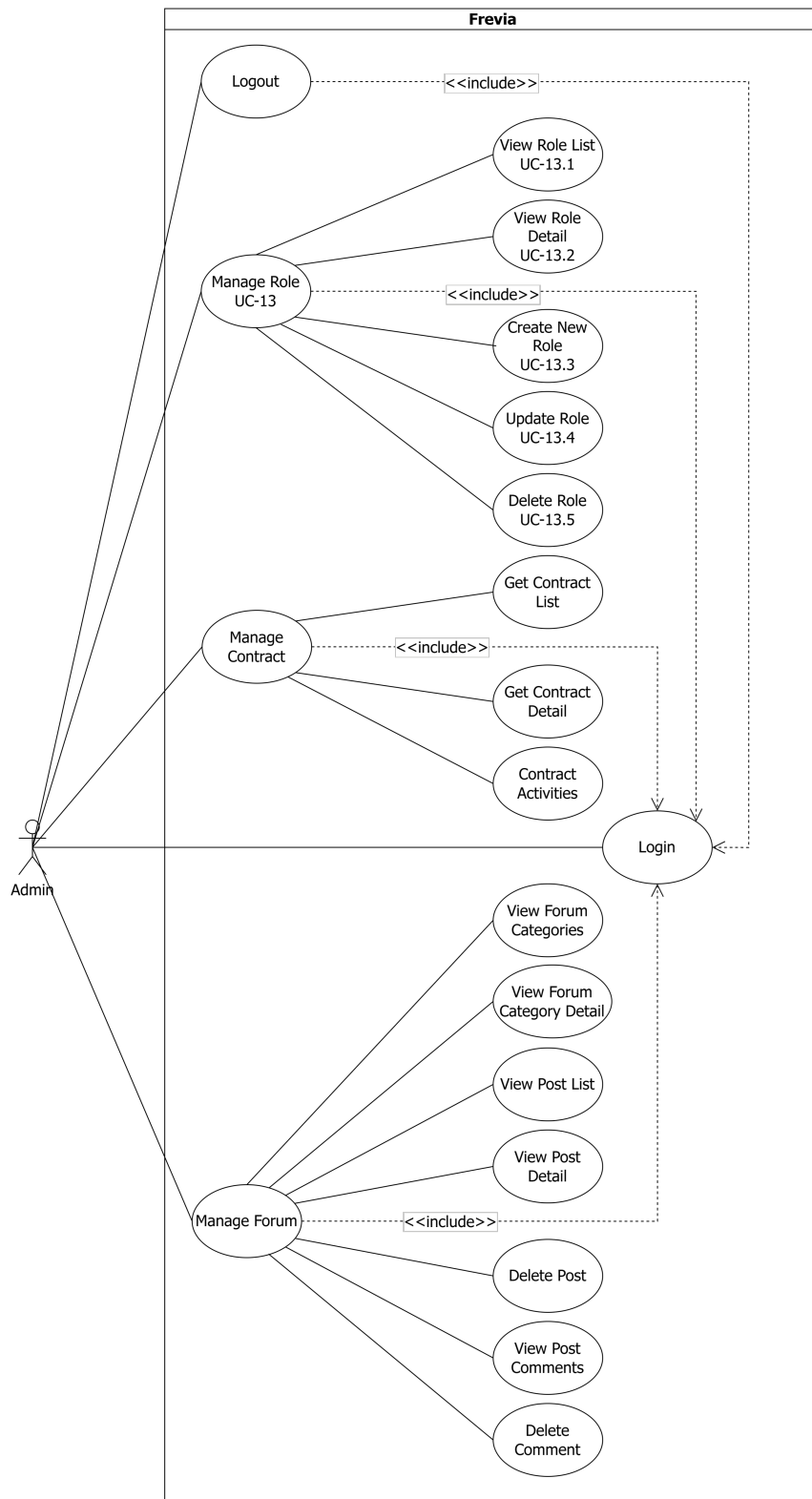
Figure 8: Admin Usecase
